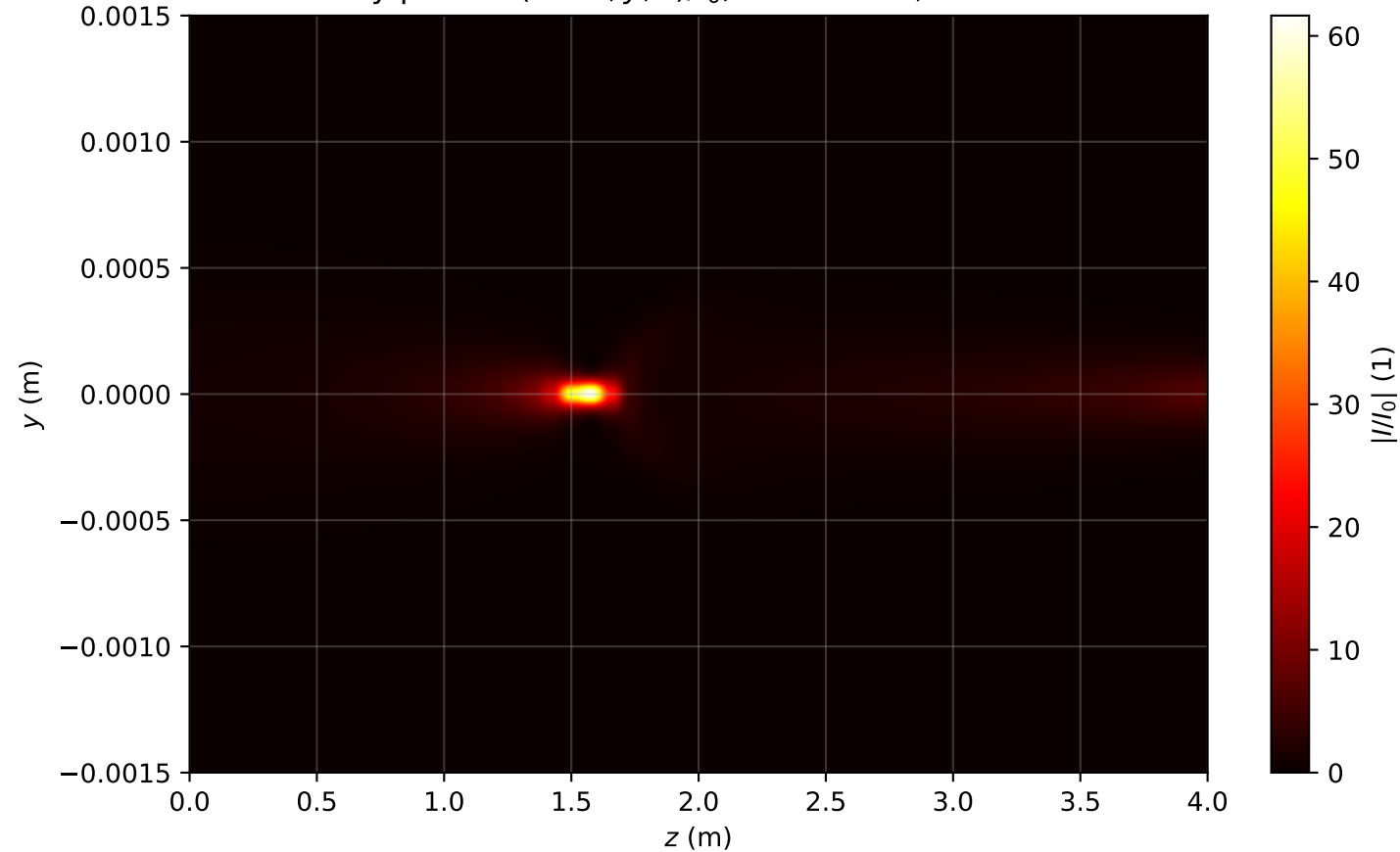
Intensity profile I(x=0, y, z)/I_0 , P_{in}=1.6P_{cr} , artificial time
